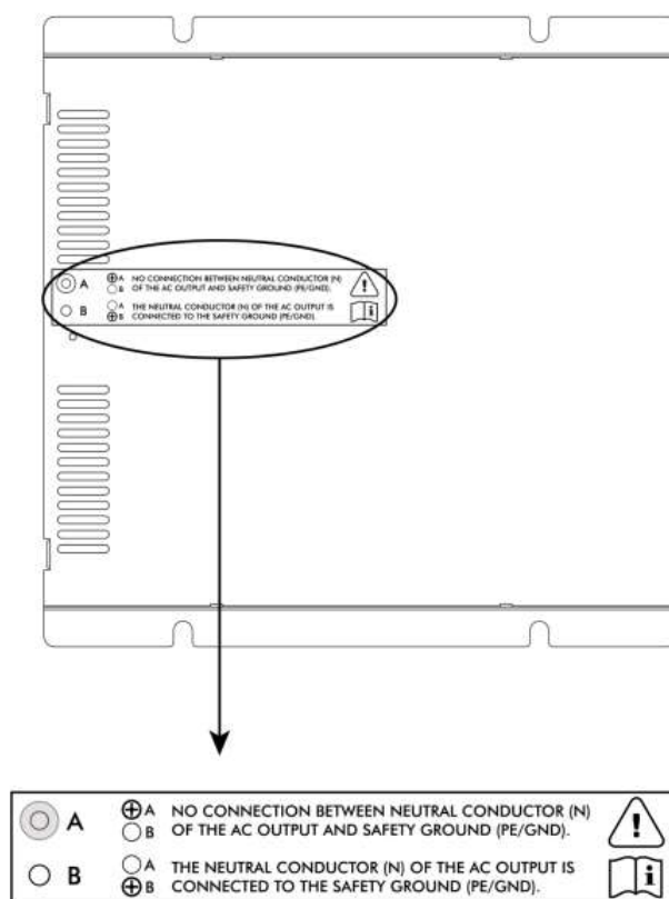
Figure 25. SD1500 Options
