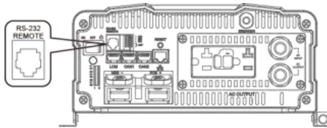
Figure 14. RS-232 port
