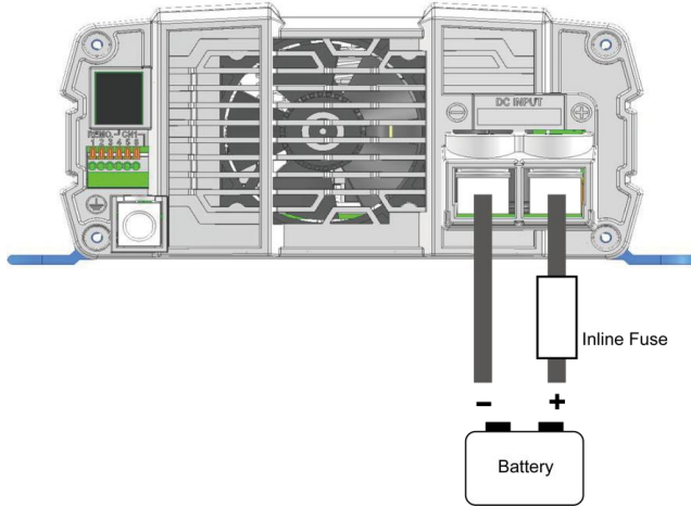
Figure 16. Battery cabling
