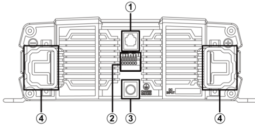
Figure 11. SP-1500/2000
