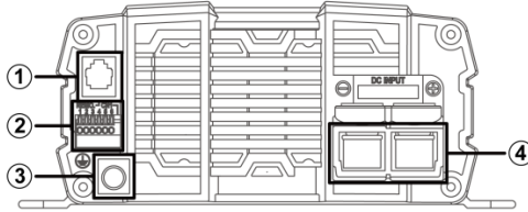
Figure 10. SP-700/1000
