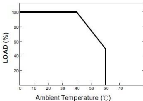
Output Derating Curve
