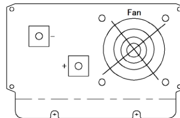
Rear panel of 300W-600W
